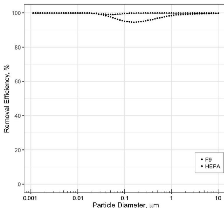
Figure 3. Single pass particle removal efficiency of a two particle filters, a HEPA filter and an F9 grade filter (according to EN779) [10]
